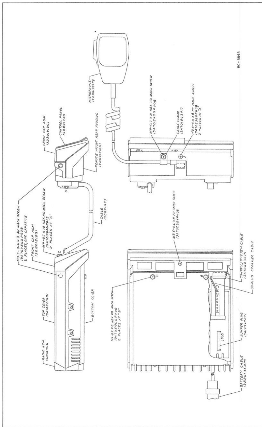
FIGURE 18 - REMOTE MOUNT INSTALLATION
